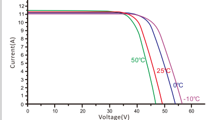
I-V characteristics at different temperatures (AM1.5, 1000W/m 2 )
