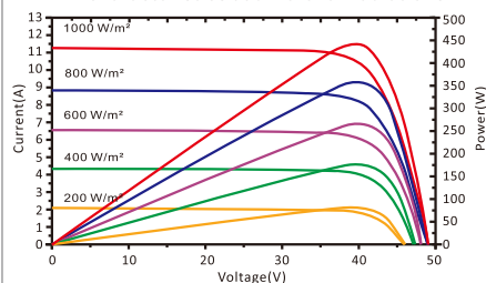
RSM144-7-440M I-V characteristics at different irradiances
